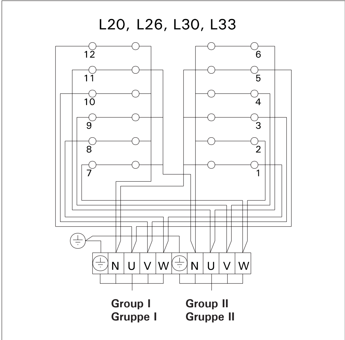
The heater's electrical connections Elektroanschlüsse des Saunaofens
