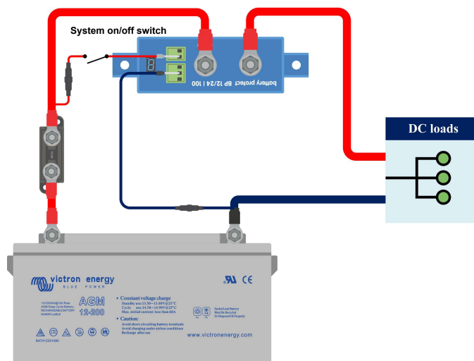
Switch wired between battery positive and the REMOTE pin of the remote terminal
