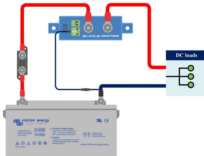
BatteryProtect in a simple system with a wire loop between the two pins of the remote terminal connector (factory default)
