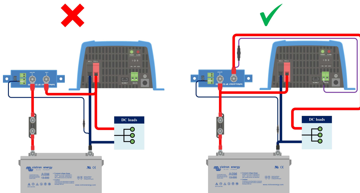
Left image: Inverter DC input connected via a BatteryProtect - strictly forbidden
