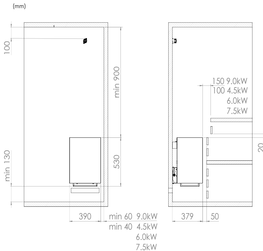
Figure 1. Safety distances
