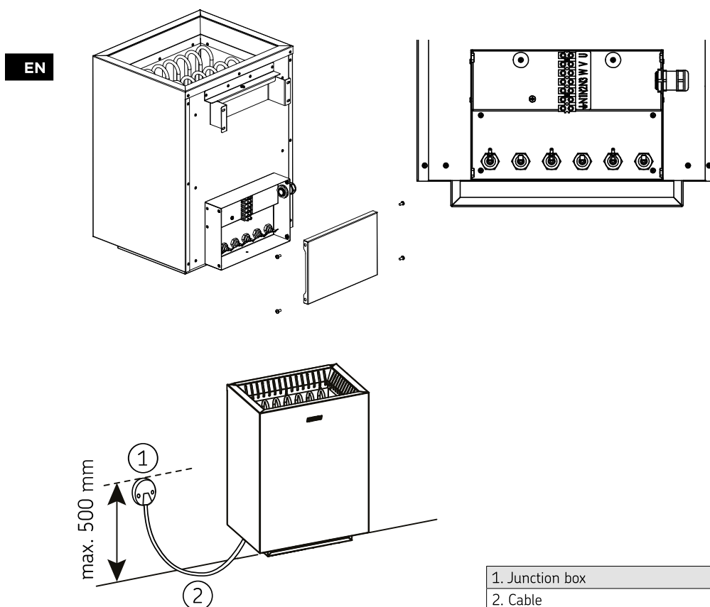
Figure 4. Electrical connections
