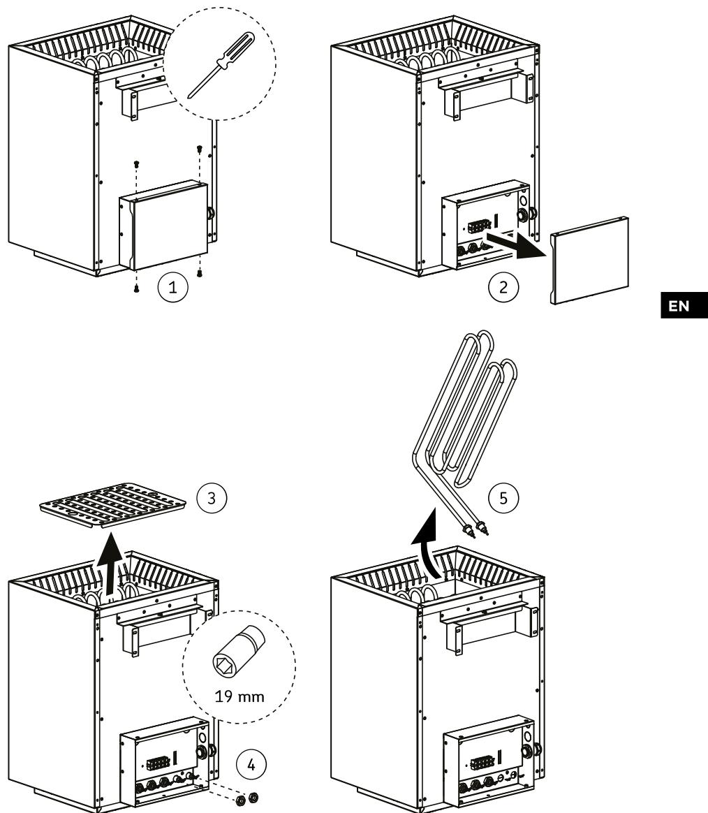
Figure 14. Changing of heating elements
