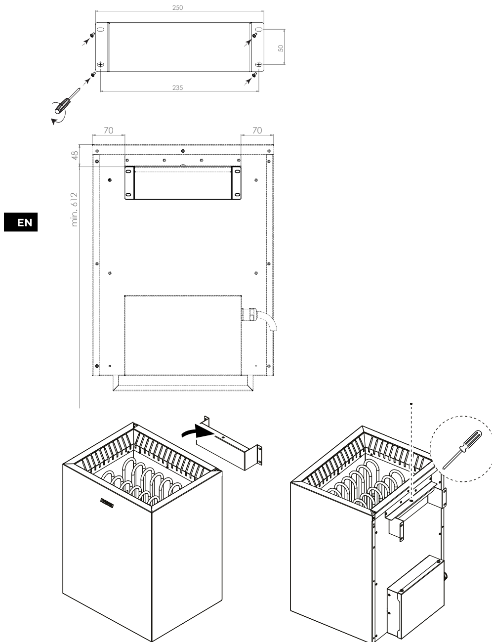
Figure 2. Sauna heater installation
