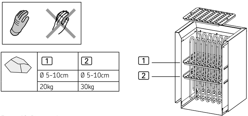
Figure 12. Placing of sauna stones
