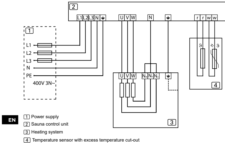
Figure 9. Connection diagram 400V 3N~
