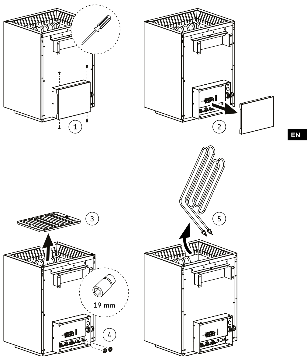
Figure 14. Changing of heating elements
