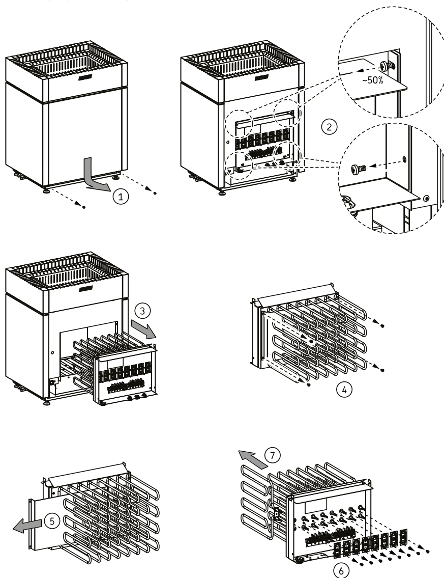
Figure 11. Changing of heating elements
