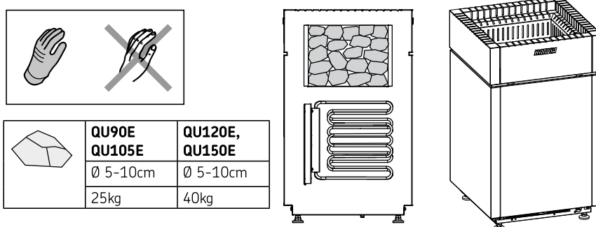
Figure 9. Placing of sauna stones
