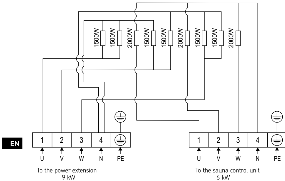
Figure 8. Wiring diagram QU150E
