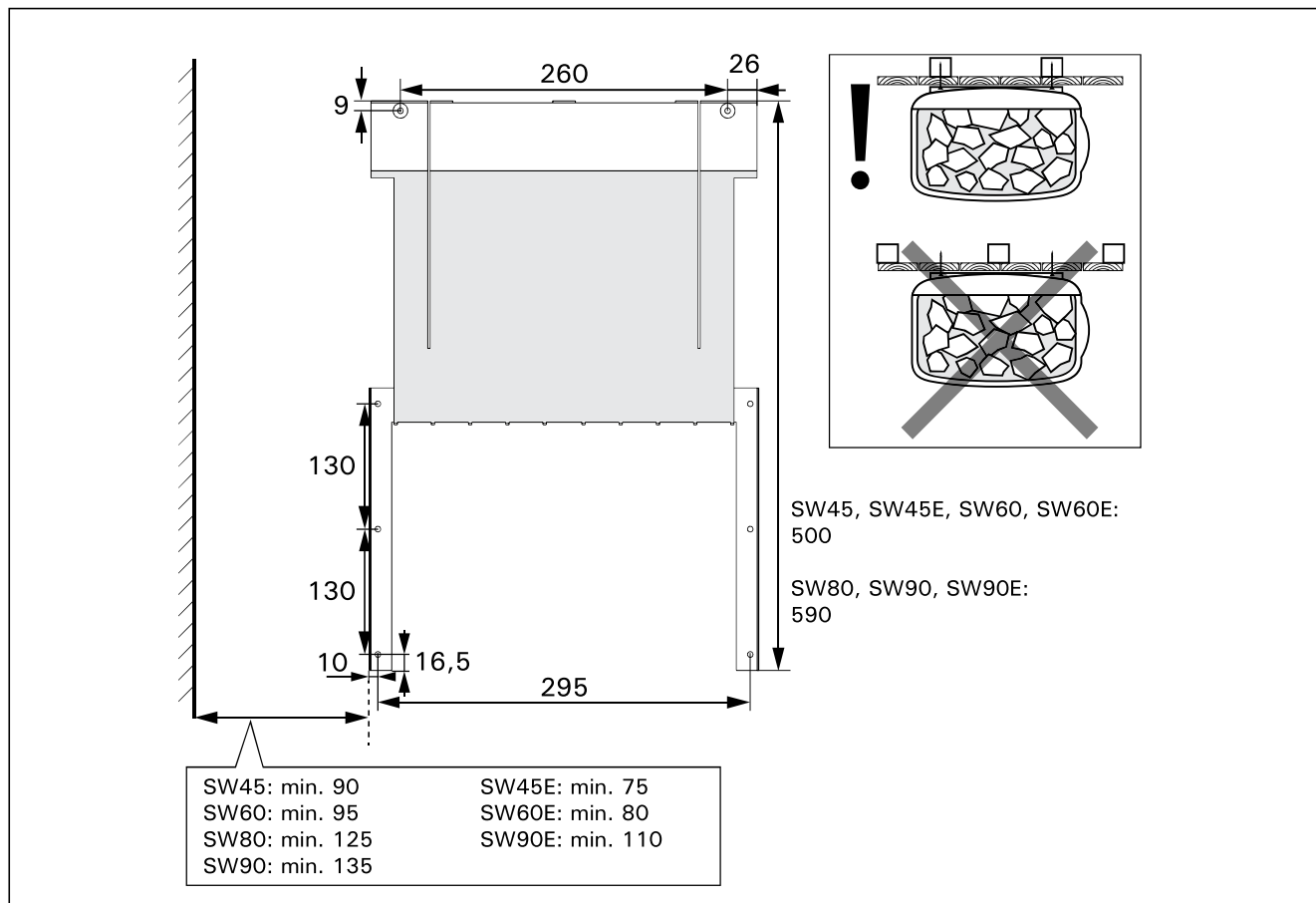
Figure 7. Support mural, dimensions en millimetres
