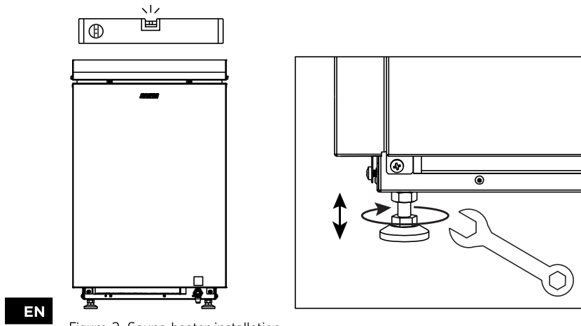
Figure 2. Sauna heater installation
