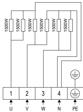
Figure 5. Wiring diagram CR90E
