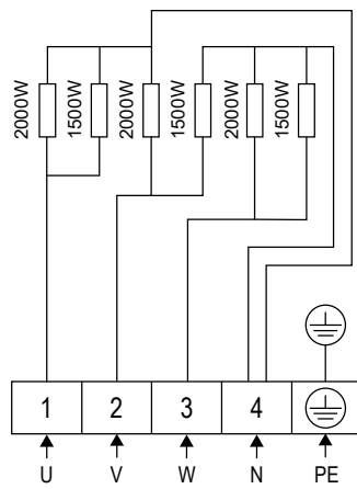
Figure 6. Wiring diagram CR105E
