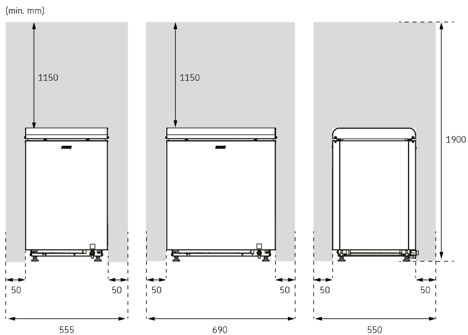
Figure 1. Safety distances
