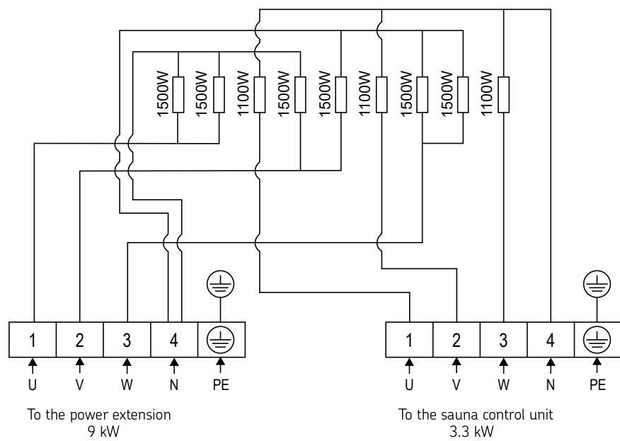
Figure 7. Wiring diagram CR120E
