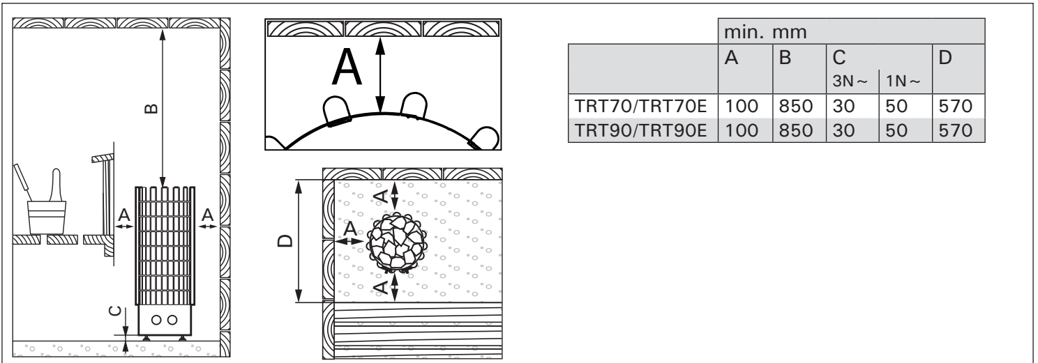
Safety distances (all dimensions in millimeters)
