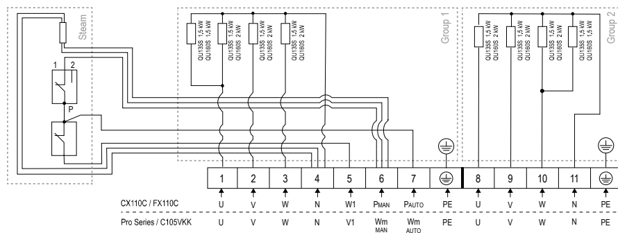
Figure 6. Wiring diagram QU135S, QU160S
