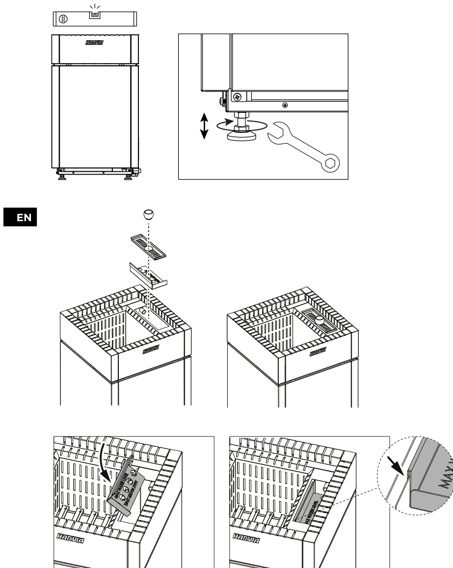
Figure 2. Sauna heater installation
