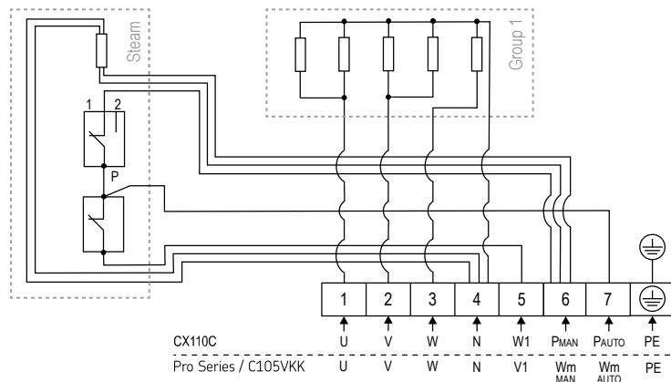
Figure 5. Wiring diagram QU100S
